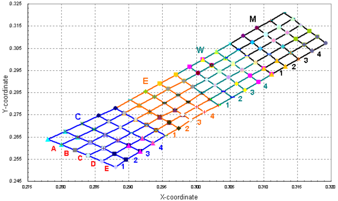
C. I. E. 1931 Chromaticity Diagram @20mA
