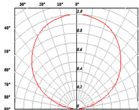
Radiation Pattern
