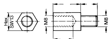
Threaded spacer for higher Anode/Cathode construction: Type ZY 250, material brass
