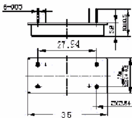
Package Outline
