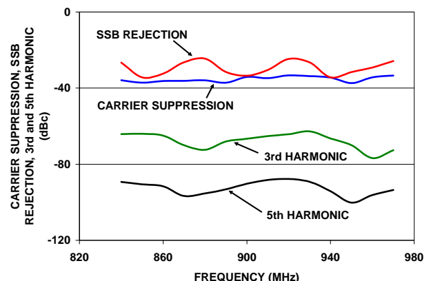
Carrier Suppression, SSB Rejection, 3rd and 5th Harmonic Suppression: V_{CC} = 3.6\text{V} , P_{LO} = +4\text{ dBm}
