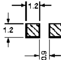
Suggested pad dimensions for reflow soldering
