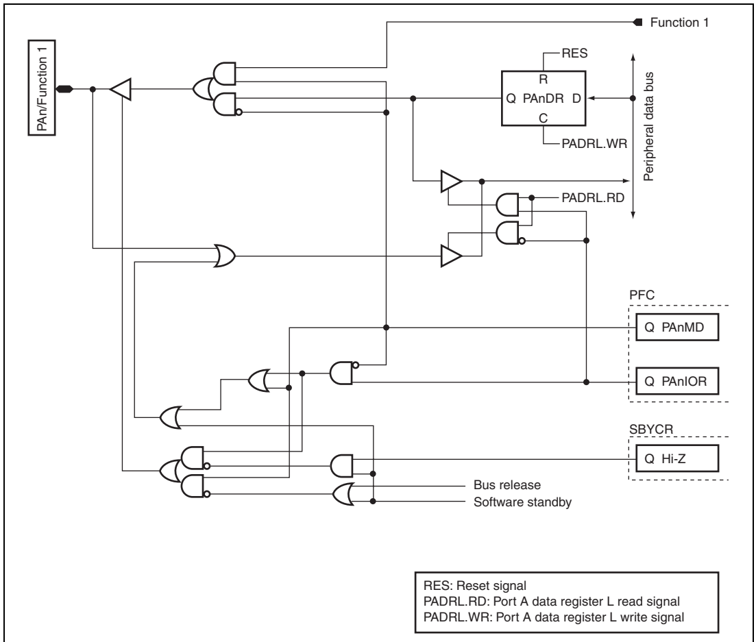
Figure D.6 PA n/Function 1
