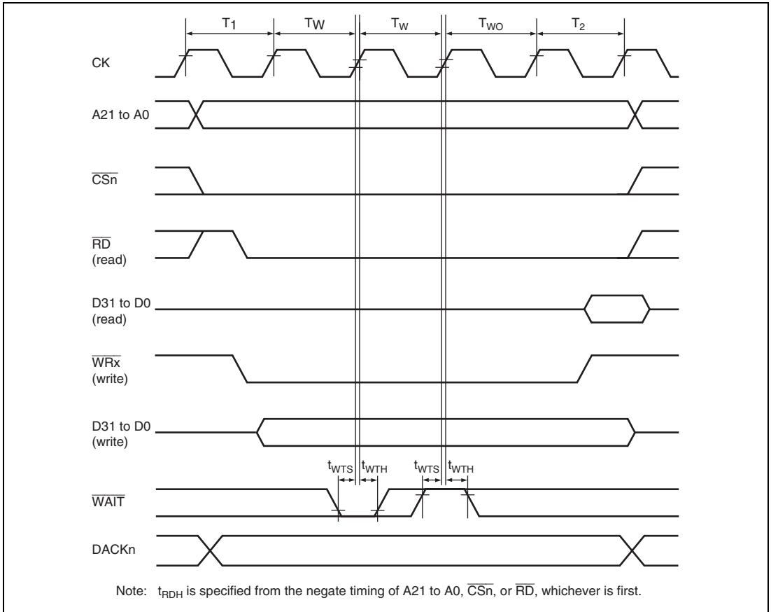
Figure 26.11 Basic Cycle (Two Software Waits + Waits by WAIT Signal)
