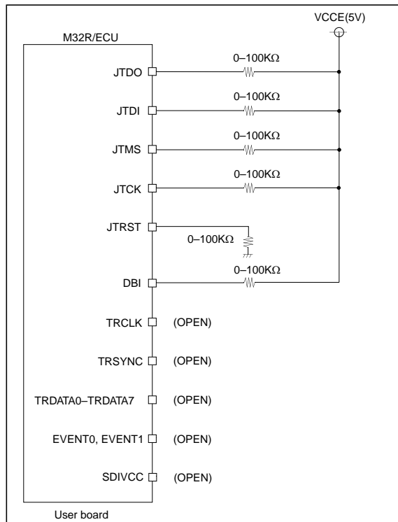
Figure 4.12.4 Processing Pins when Not Using JTAG (for 255FBGA)
