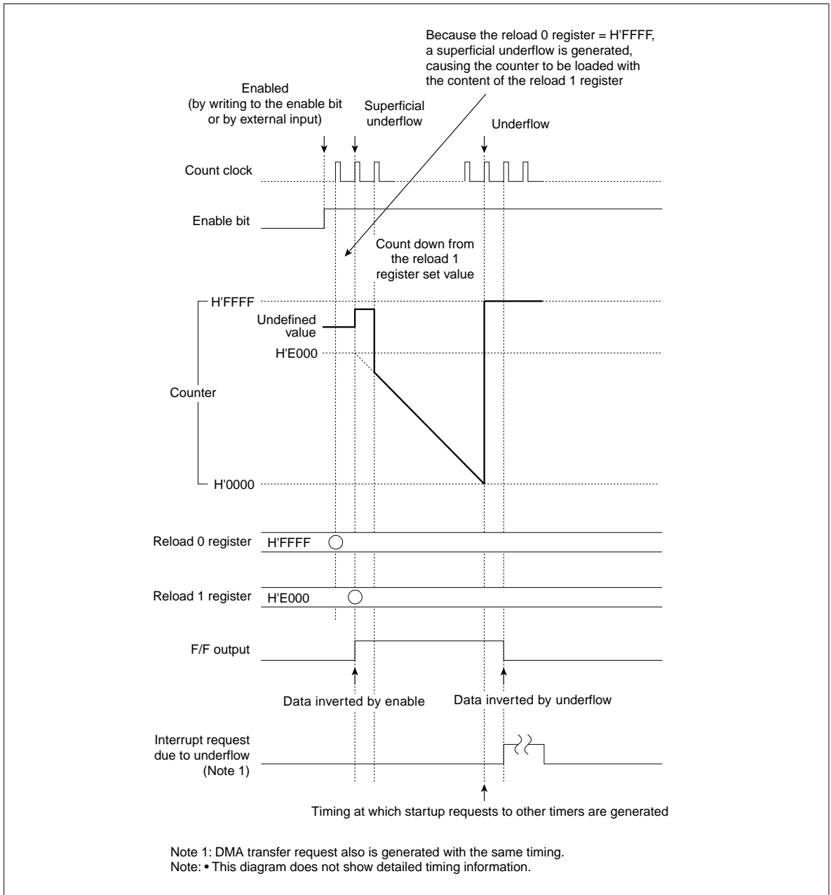
Figure 10.8.19 Typical Operation in Single-shot PWM Output Mode (Reload 0 Register: H'FFFF)
