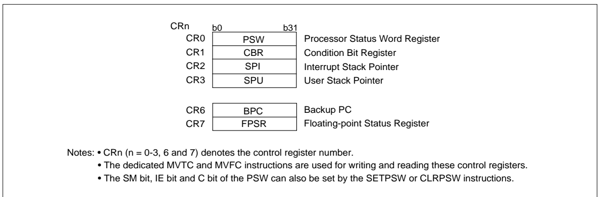
Figure 2.3.1 Control Registers
