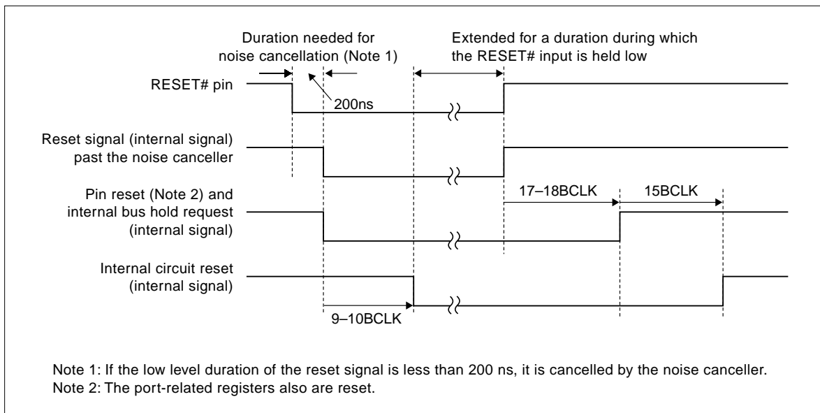
Figure 7.2.2 Reset Sequence
