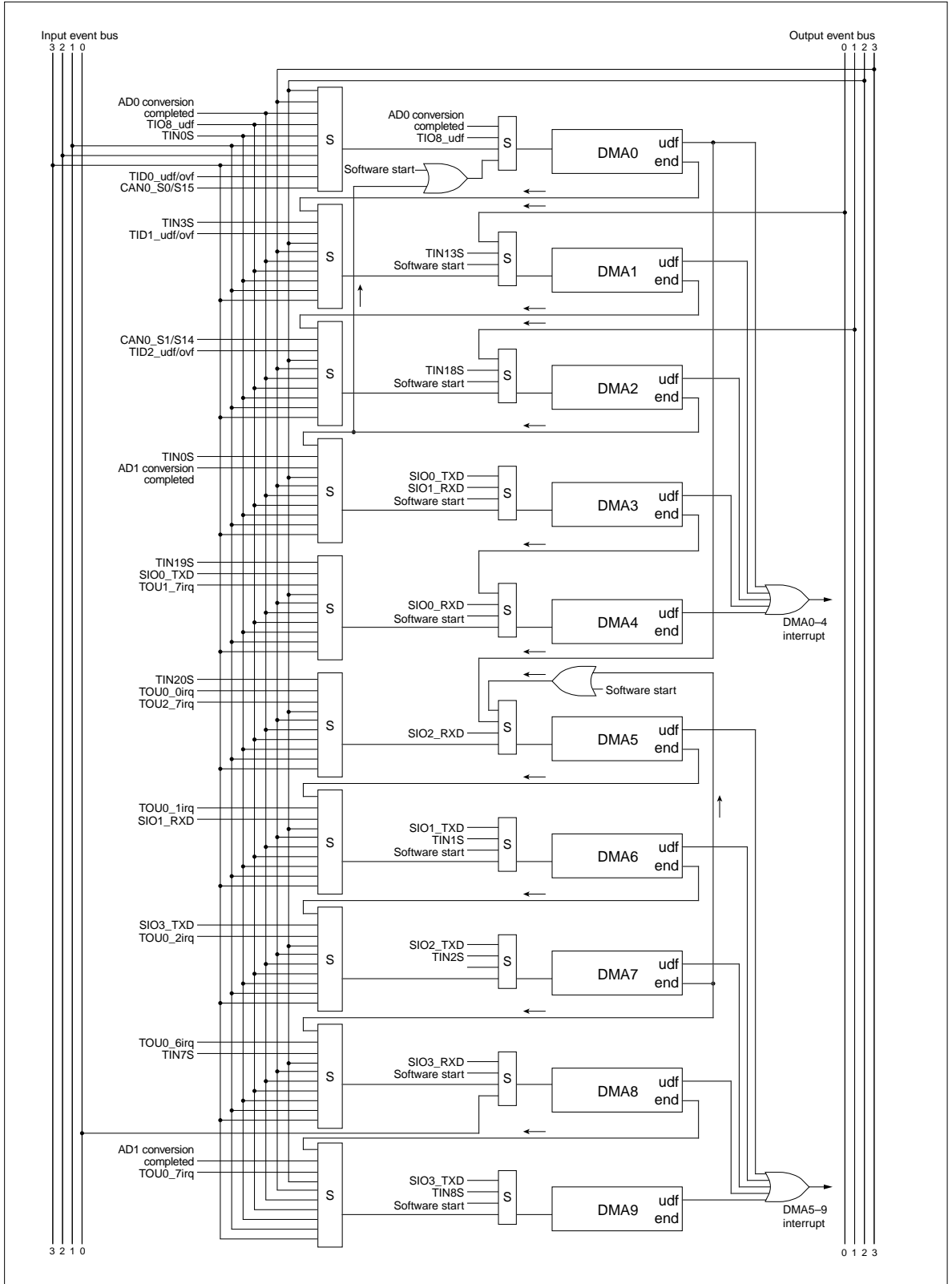
Figure 10.1.4 Block Diagram of MJT (4/4)
