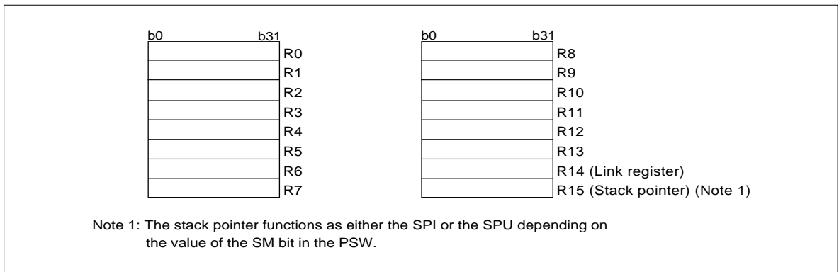
Figure 2.2.1 General-purpose Registers
