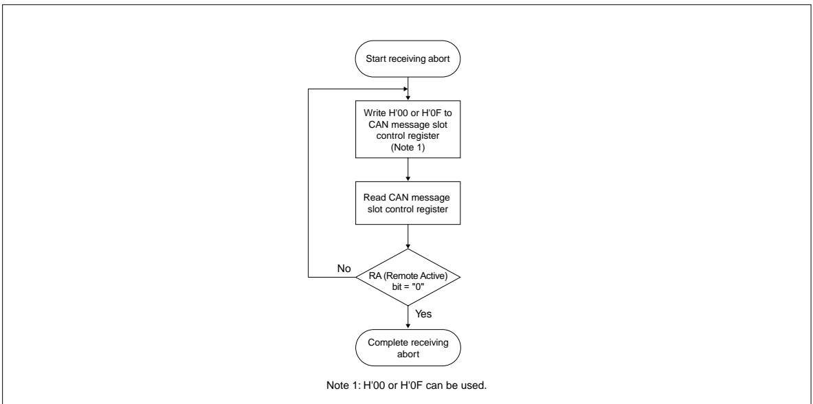
Figure 13.9.2 Operation Flow when Canceling Remote Frame Receiving
