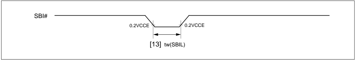
Figure 21.7.3 SBI Timing
