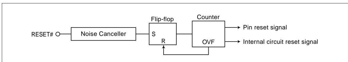
Figure 7.2.1 Reset Circuit
