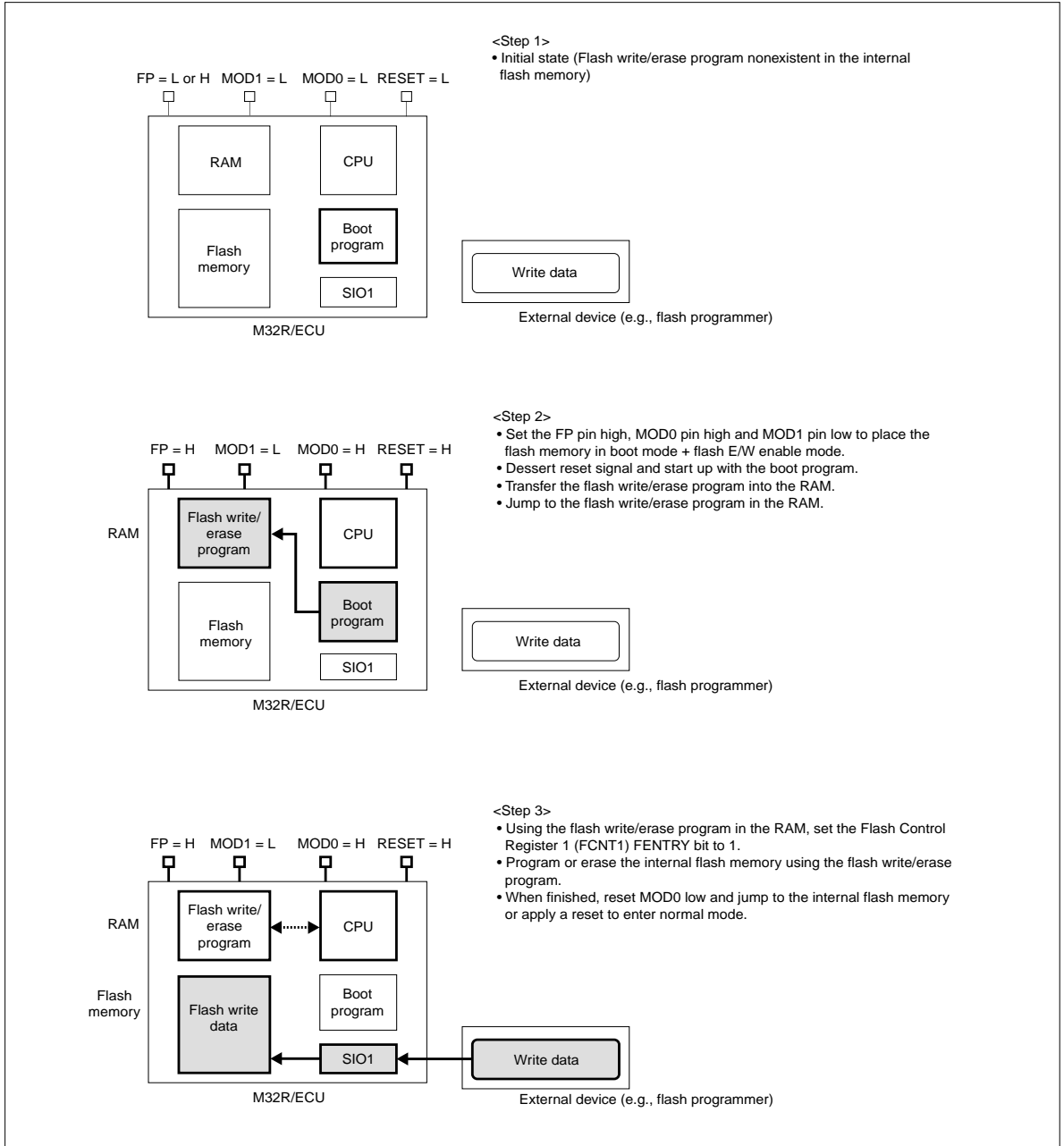
Figure 6.5.2 Procedure for Programming/Erasing the Internal Flash Memory (when the flash write/erase program does not exist in it)
