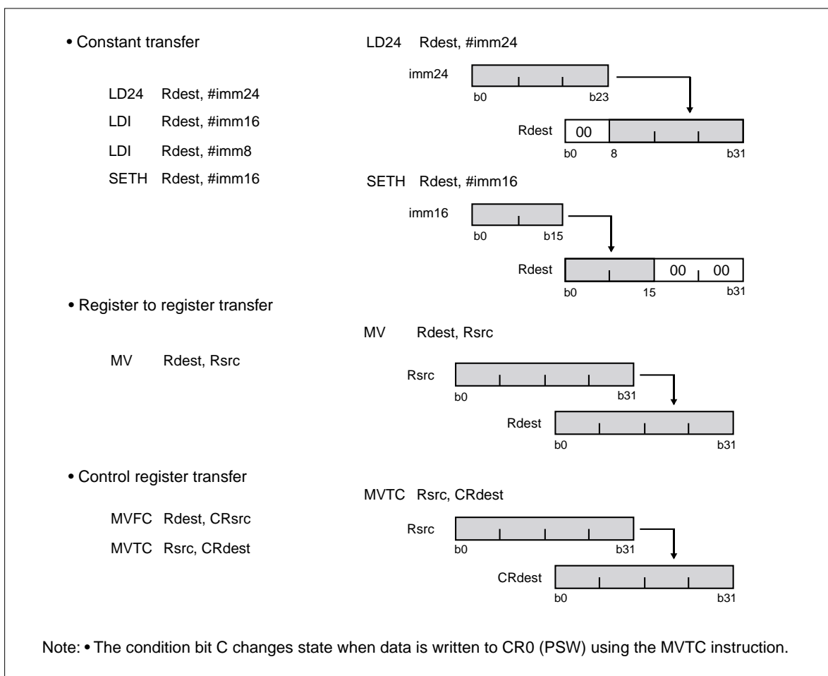
Figure 2.6.6 Transfer Instructions
