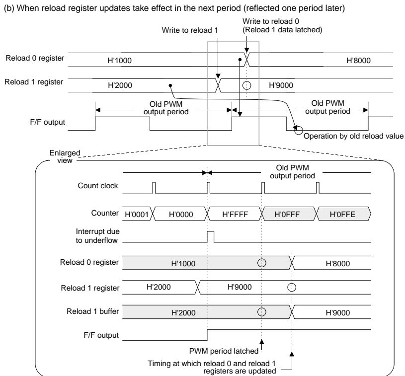
Figure 10.4.11 Reload 0 and Reload 1 Register Updates in PWM Output Mode
