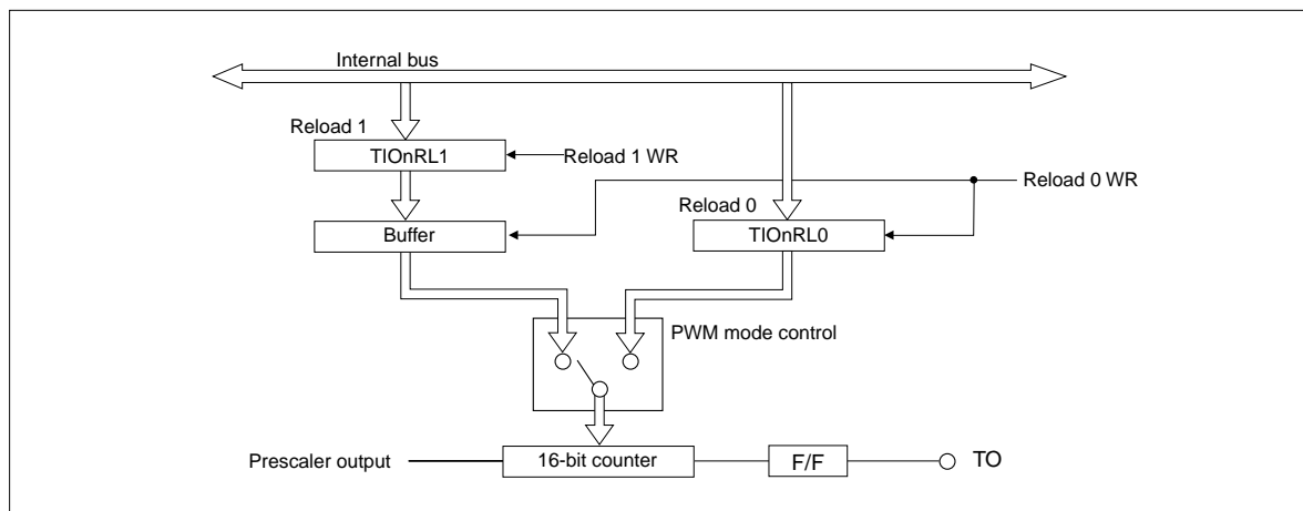
Figure 10.4.10 PWM Circuit Diagram
