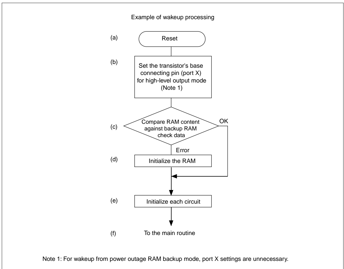
Figure 17.4.1 Wakeup Processing
