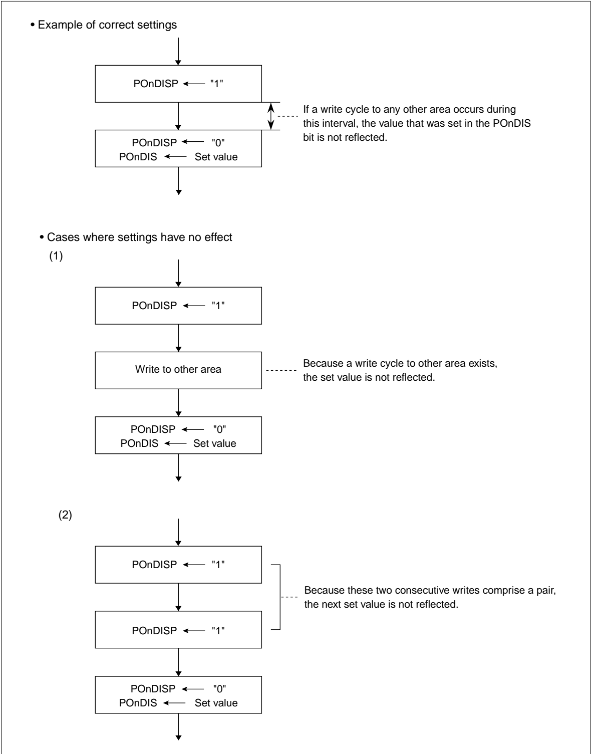
Figure 10.8.8 POnDIS Setting Procedure
