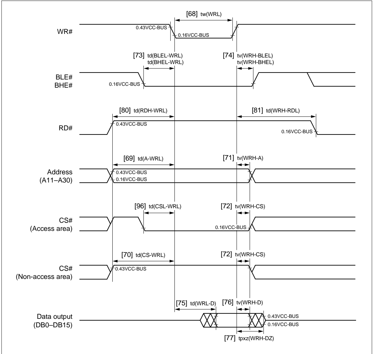
Figure 21.8.10 Write Timing (Byte Enable Mode)
