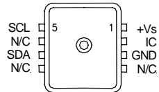
CSDX...A2R, CSDX...BARO
