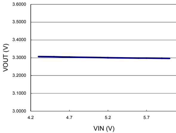
Line Regulation ( V_{OUT} = 3.3V ) ( V_{IN} = 4.3V to 6V , I_{OUT} = 1mA )
