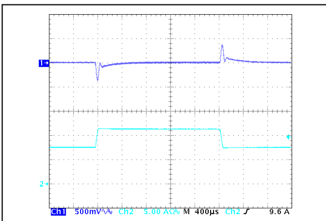
Figure 5: Output voltage response to step-change in load current (50%-75%-50% of I out (max)); di/dt = 0.1 \text{ A}/\mu\text{s} . Load cap: 1 \mu\text{F} ceramic capacitor. Ch 1: V out (500 mV/div), Ch 2: I out (5 A/div).
