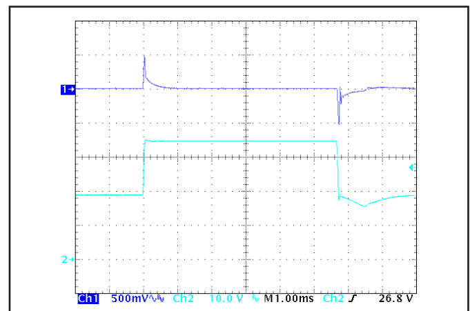
Figure 6: Output voltage response to step-change in input voltage (1000 V/ms). Load cap: 100 \mu\text{F} , electrolytic output capacitance. Ch 1: V out (500 mV/div), Ch 2: V in (10 V/div).
