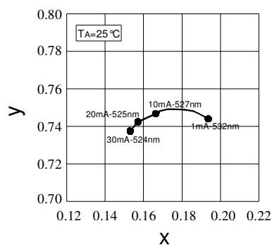
Forward Current vs. Chromaticity Coordinate
