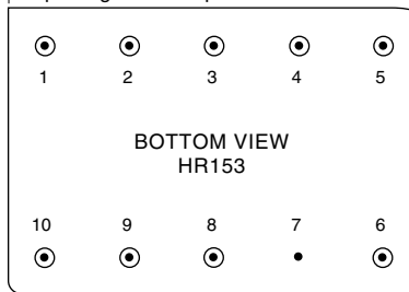
FIGURE 2: HR153 PIN OUT
