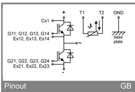
Case SEMiX 4s
