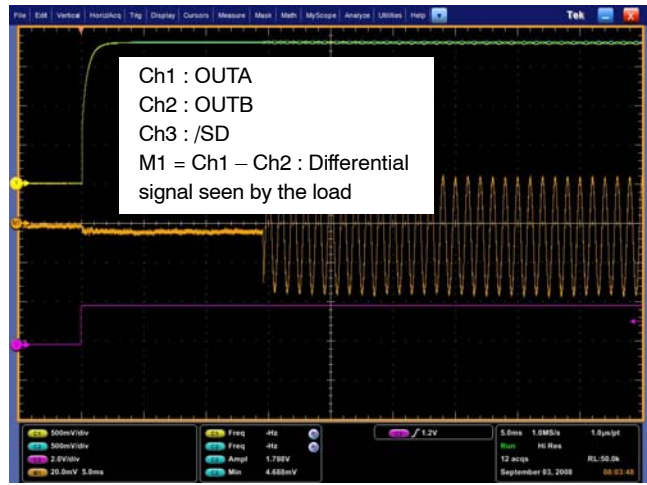
Figure 34. Zero pop noise turn on sequence with single-ended input audio source ( C_i = 47\text{ nF} , R_i = 24\text{ k}\Omega , R_f = 24\text{ k}\Omega , C_{byp} = 1\text{ }\mu\text{F} , R_l = 8\text{ }\Omega , T_{on} = V_p )
