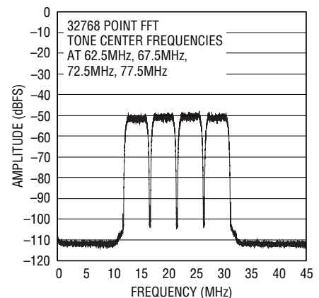
4-Tone WCDMA Waveform LT1993-10 Driving LTC2255 14-Bit ADC at 92.16Mps
