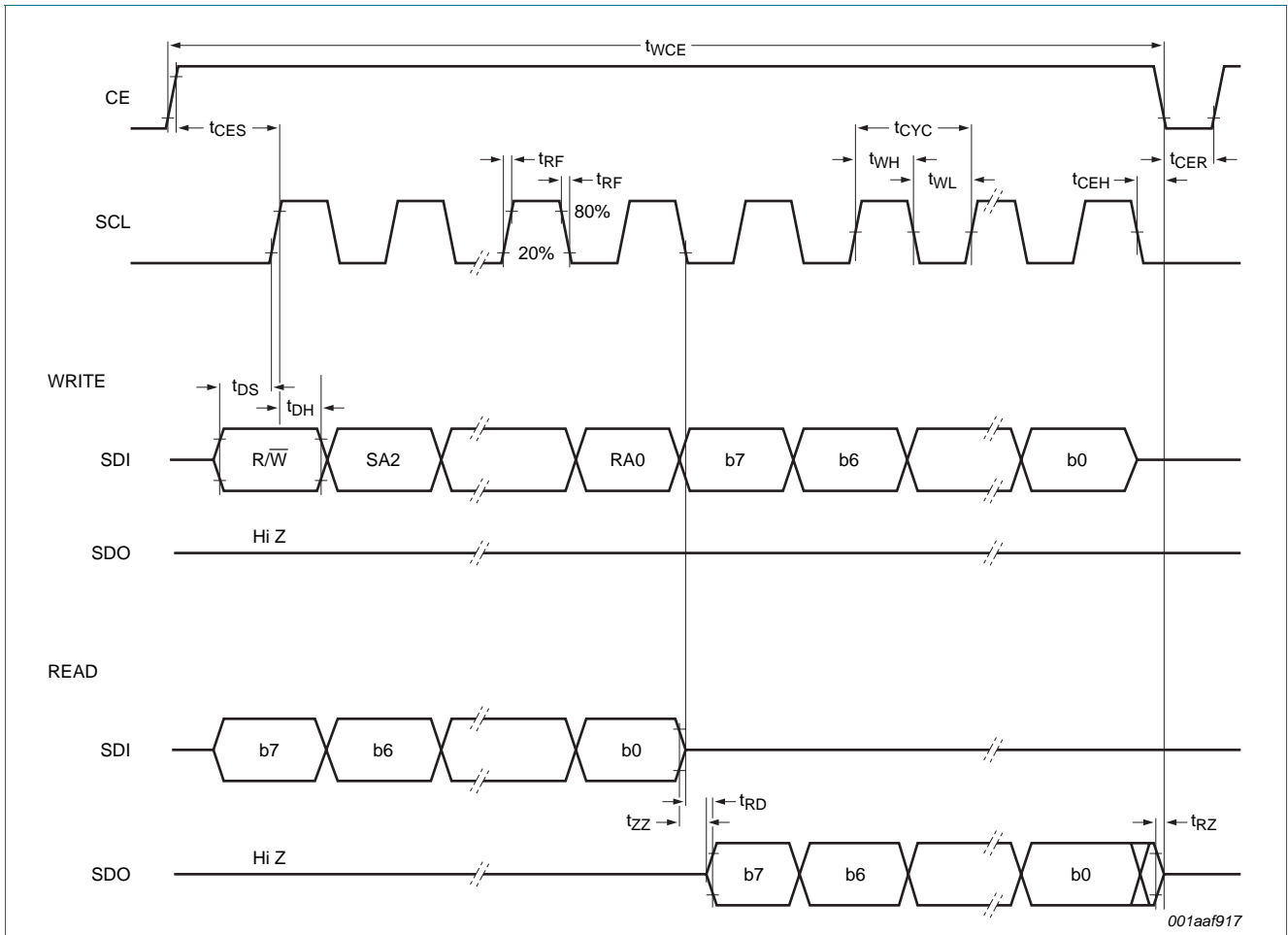
Fig 21. SPI interface timing
