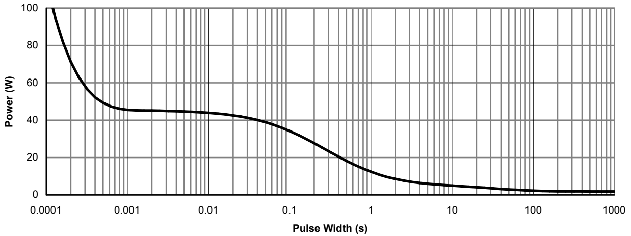
Figure 15: Single Pulse Power Rating Junction-to-Ambient (Note H)
