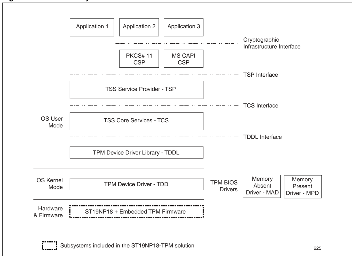
Figure 2. Software layers
