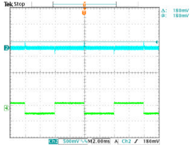
Figure 16. Output voltage dynamic response at Vin=48v Iout= 12~20A, 2.5A/us dynamic load. waveform 2 is dynamic response via dynamic load. waveform 4 is load current (2.5A/us); with 220uF output capacitance load.
