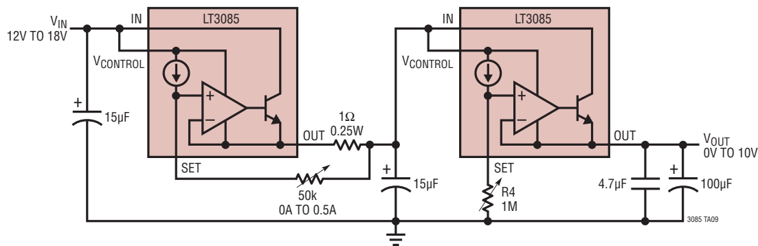
Lab Supply
