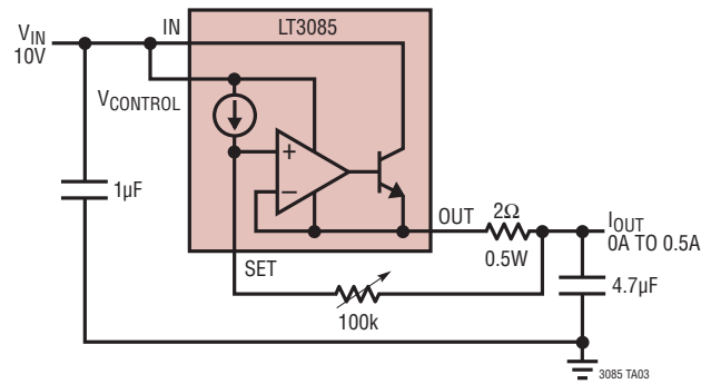
Current Source
