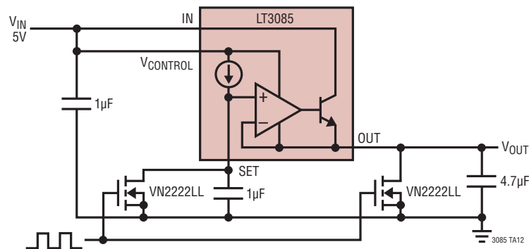
Ramp Generator
