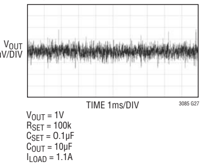
Output Voltage Noise
