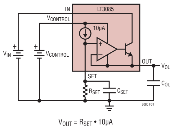
Figure 1. Basic Adjustable Regulator
