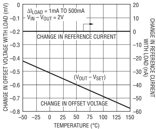
Load Regulation
