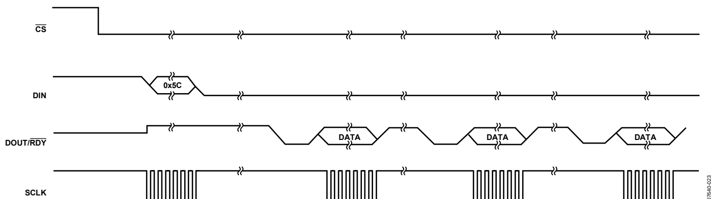
Figure 31. Continuous Read
