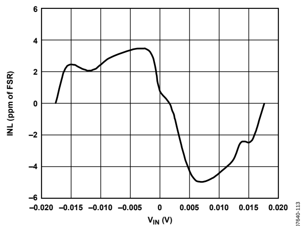
Figure 13. INL (Gain = 128)
