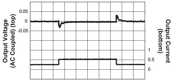
Load Transient
