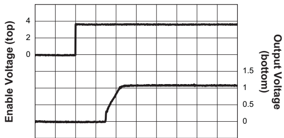
Soft-Start
