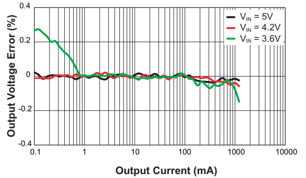
Load Regulation ( V_{OUTB1} = 3.3V ; L = 3.3\mu H )
