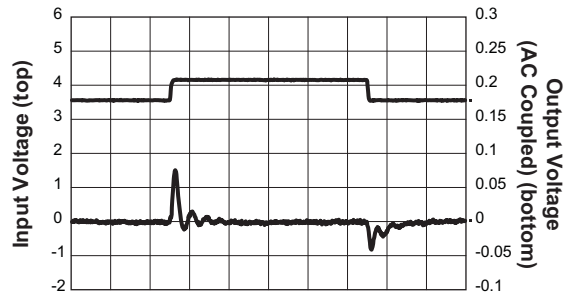
Line Transient
