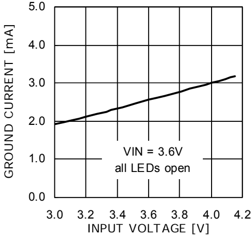
Ground Current vs. Input Voltage (1.5x mode)
