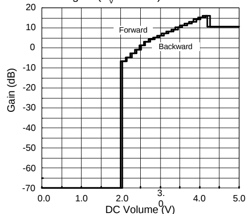
Figure 4: APA2057A Gain setting vs. SET pin Voltage
