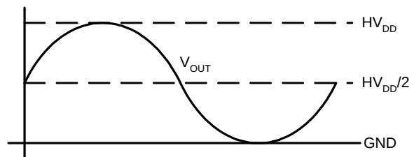
Conventional Headphone amplifier
