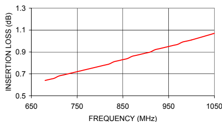
TCN1-10 INSERTION LOSS
