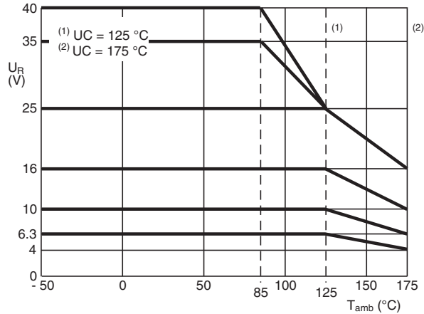
Fig.3 Maximum permissible voltage up to 175 °C
