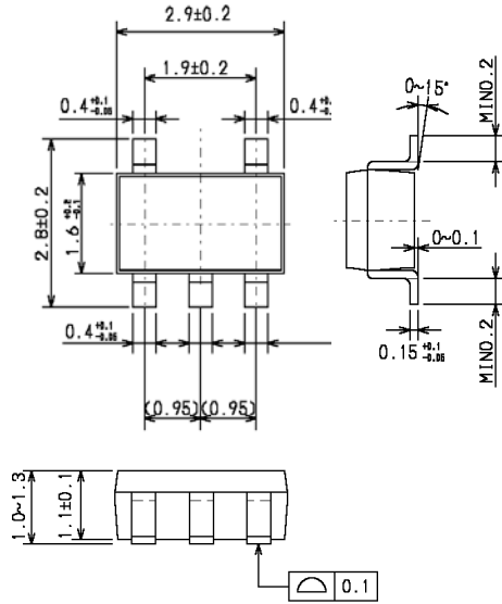
SOT-25 (SOT-23-5)
