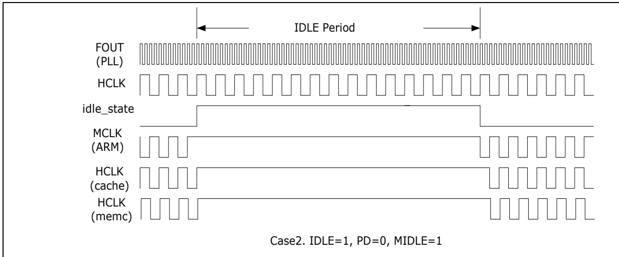
Fig. 7.2.8 Clock management for system and memory idle mode
