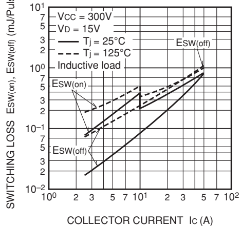
SWITCHING LOSS CHARACTERISTICS (Lower Arm · TYPICAL)
