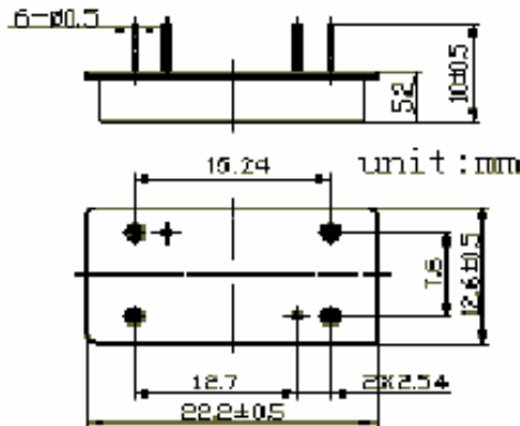
Package Outline
