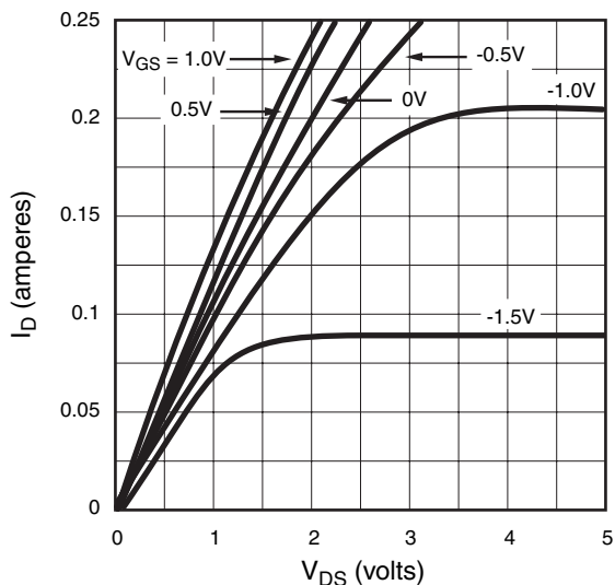
Saturation Characteristics
