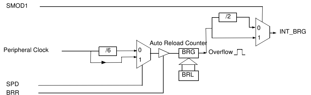
Figure 5. Internal Baud Rate Generator
