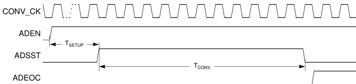
Figure 2. Timing Diagram
