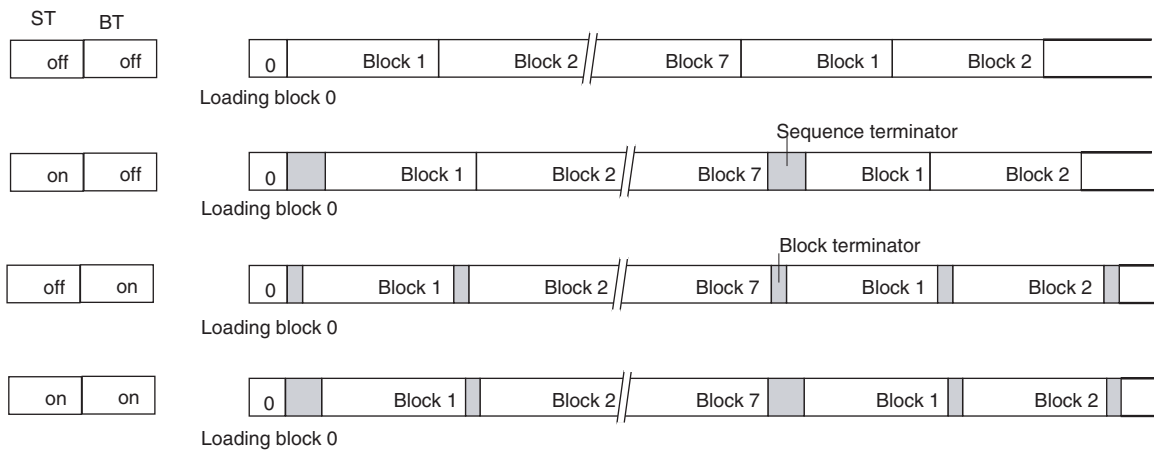
Figure 4-4. Read Data Streams and Terminators
