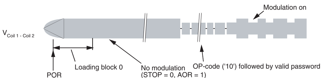
Figure 4-6. Answer-on-request (AOR) Mode
