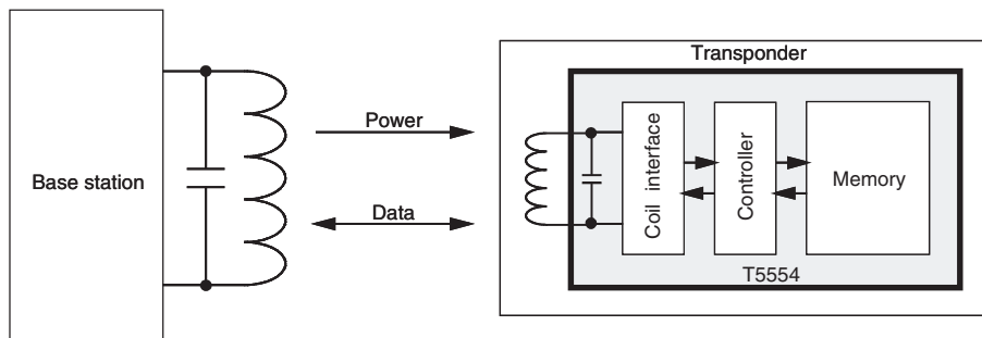
Figure 2-1. RFID System Using T5554 Tag
