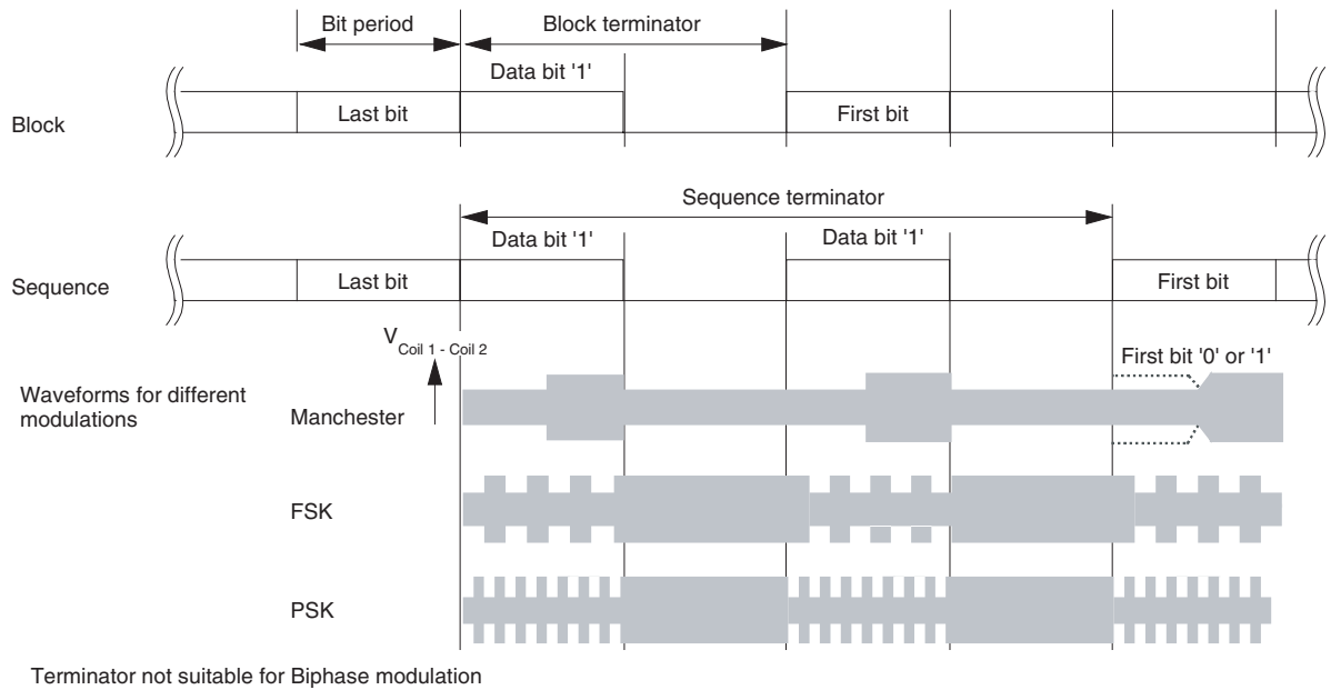
Figure 4-3. Terminators
