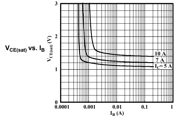
STD02N Performance Characteristics at T_A = 25^\circ\text{C}
