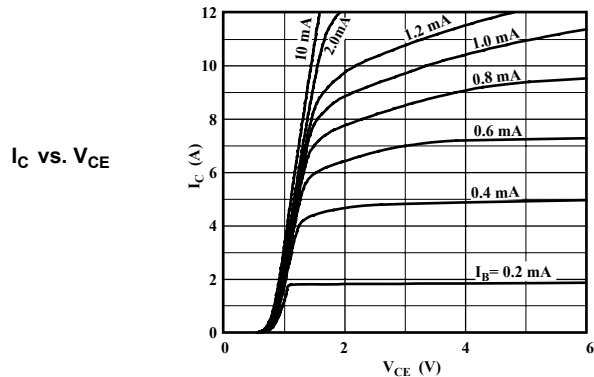
STD02N Performance Characteristics at T_A = 25^\circ\text{C}
