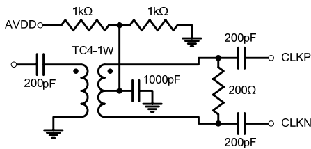
Figure 33. Recommended Clock drive
