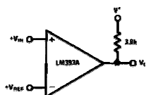
Basic Comparator
