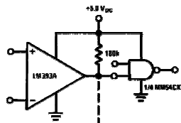
Driving CMOS
