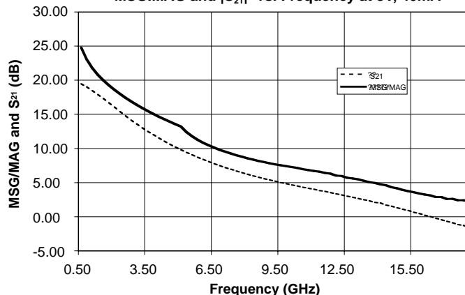
MSG.MAG and |S_{21}|^2 vs. Frequency at 3V, 40mA
