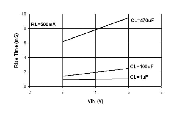
Figure 25. Output rise time vs. V_{IN}
