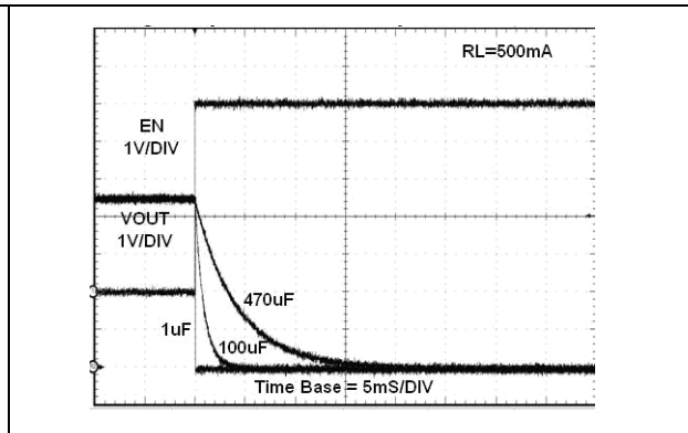
Figure 4. Voltage output turn off delay time
