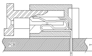
PCB ASS'Y (FCZ254-NNR)
