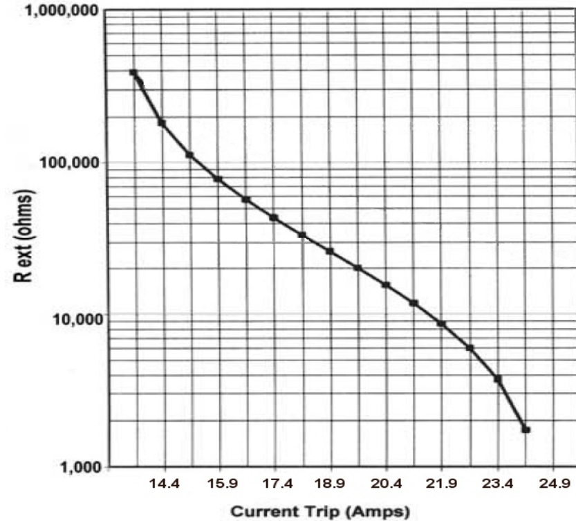
Figure 6 – SPDP03D375 Instant Trip Trim Resistor Selection
