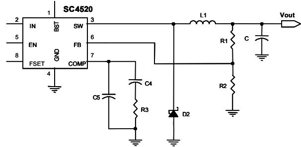
Figure 3. Compensation network provides 2 poles and 1 zero.
