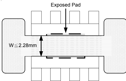
Figure 9. Dog-Bone layout
