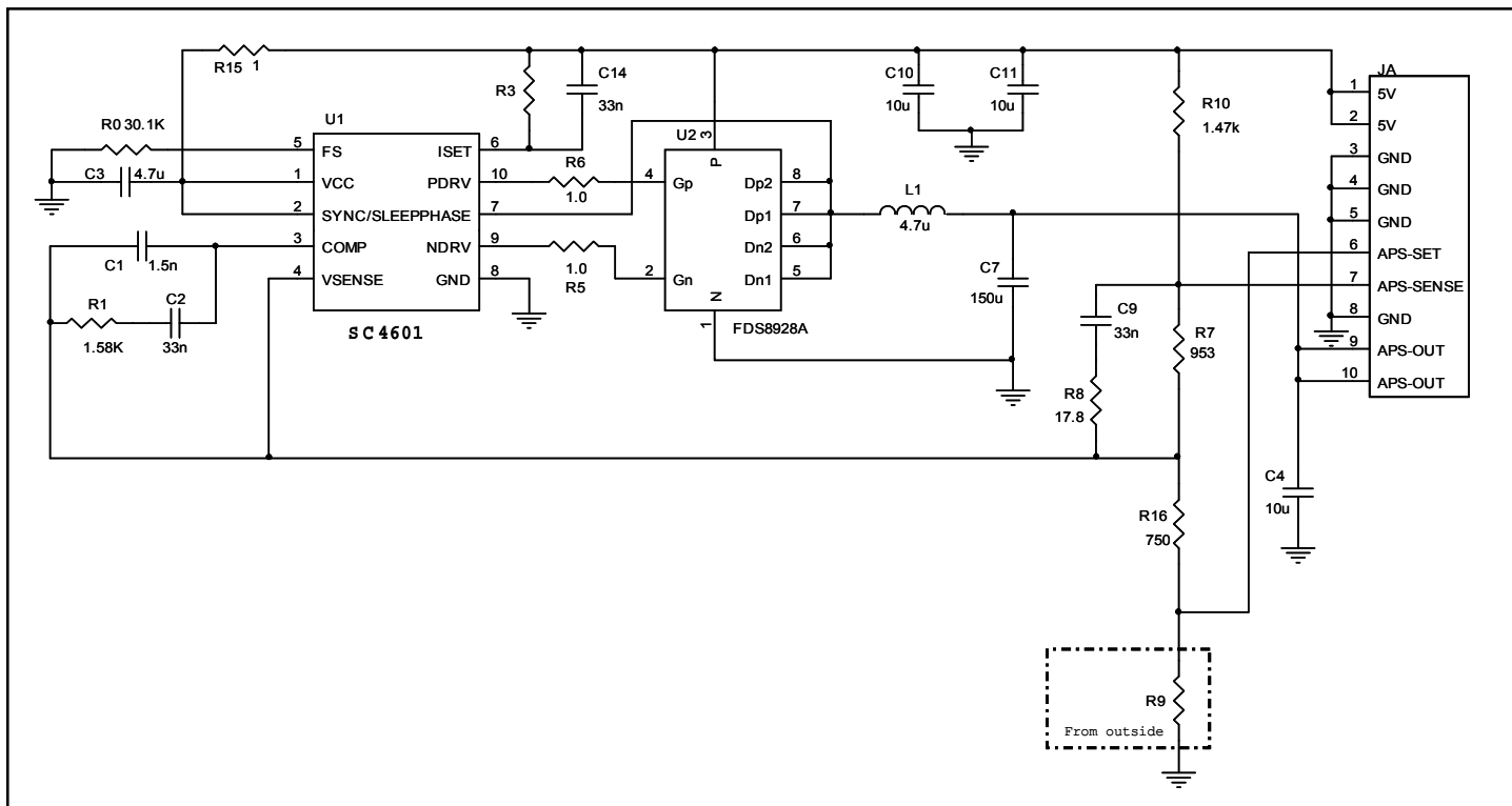
Figure 7. Schematic for Xepak application with SC4601
