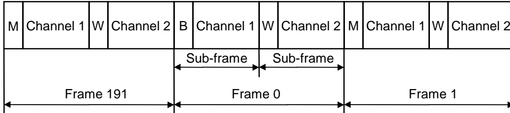
Figure 14. Block format
