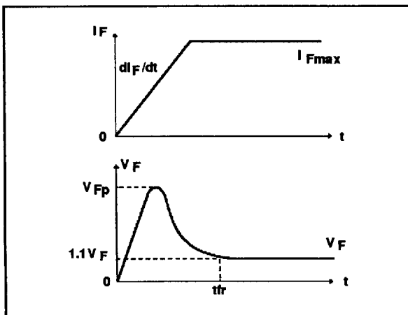
Fig. 7: TURN-ON CHARACTERISTICS
