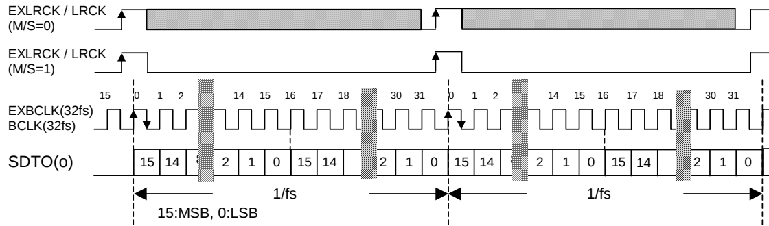
Figure 26. Mode 0 Timing (BCKP = "0", MSBS = "0", M/S = "0" or "1")
