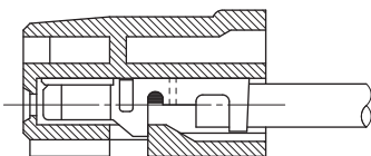
TERMINAL ASSEMBLY DRAWING
