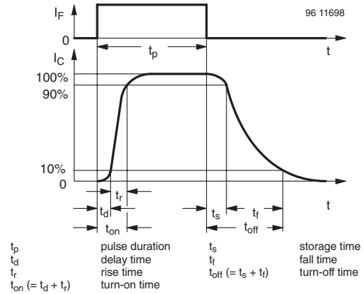
Figure 2. Switching Times
