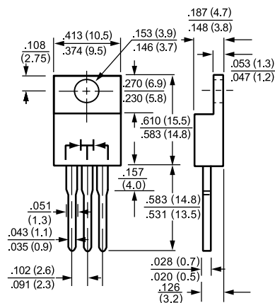
TO-220
